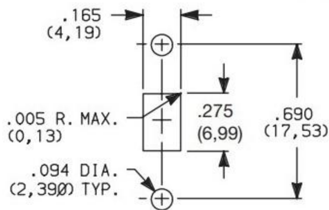
All actuators except T3. Single pole
